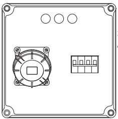
Drawing No. AS157 JEPJB300 - BOX 32 Amps 3Pin+Earth+Neutral Angular Socket IP-67 & Indicator Provision for 4 Pole MCB
