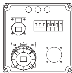
Drawing No. AS137 JEPJB300 - BOX 63 Amps 3Pin+Earth+Neutral Angular Socket IP-67 16 Amps 2Pin+Earth Angled Socket IP-67 & Indicator Provision for 32 Amps 3Pin+Earth+Neutral Straight Socket IP-44 Provision for 3+3+1 Pole MCB
