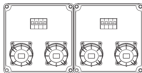
Drawing No. AS094 JEPJB300 - BOX - 2 Nos. 32 Amps 3Pin+Earth+Neutral Angular Socket IP-67 (4 Nos)
