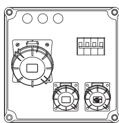
Drawing No. AS104 JEPJB300 - BOX 63 Amps 3Pin+Earth+Neutral Angular Socket IP-67 16 Amps 2Pin+Earth Angled Socket IP-67 & Indicator Provision for 4 Pole MCB
