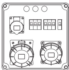
Drawing No. AS121 JEPJB300 - BOX 63 Amps 3Pin+Earth+Neutral Angular Socket IP-67 32 Amps 3Pin+Earth+Neutral Angular Socket IP-67 16 Amps 2Pin+Earth Angled Socket IP-44 & Indicator
